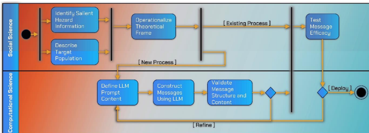
Figure 2. UML Activity Diagram Modelling the Flow of Activities in an Instantiation of the DARC Framework.
